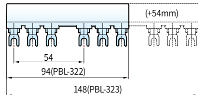
MMS-32H,HI+PBL-32 PBL-322(2 단자용), PBL-323(3 단자용)
