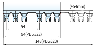
MMS-32S+PBL-32 PBL-322(2 단자용), PBL-323(3 단자용)
