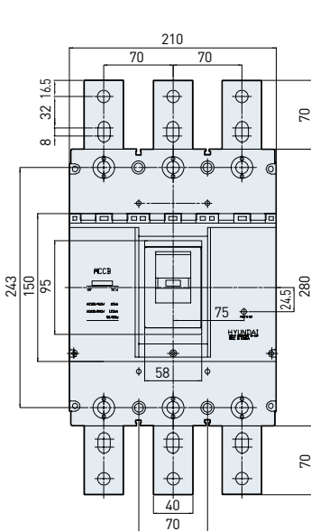
[Terminal part]
