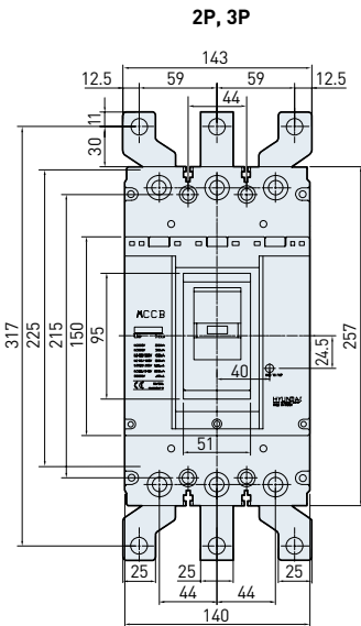
[Terminal part]
