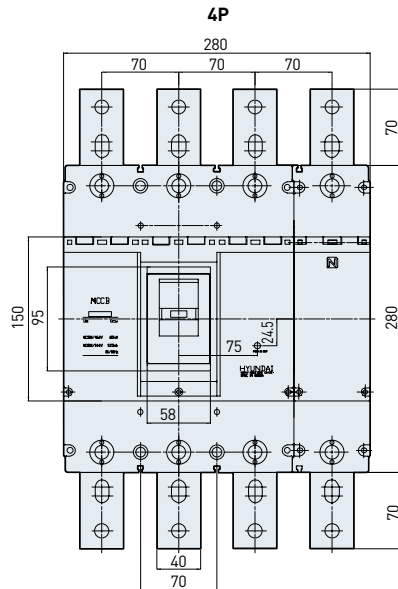
[Connection conductor]
