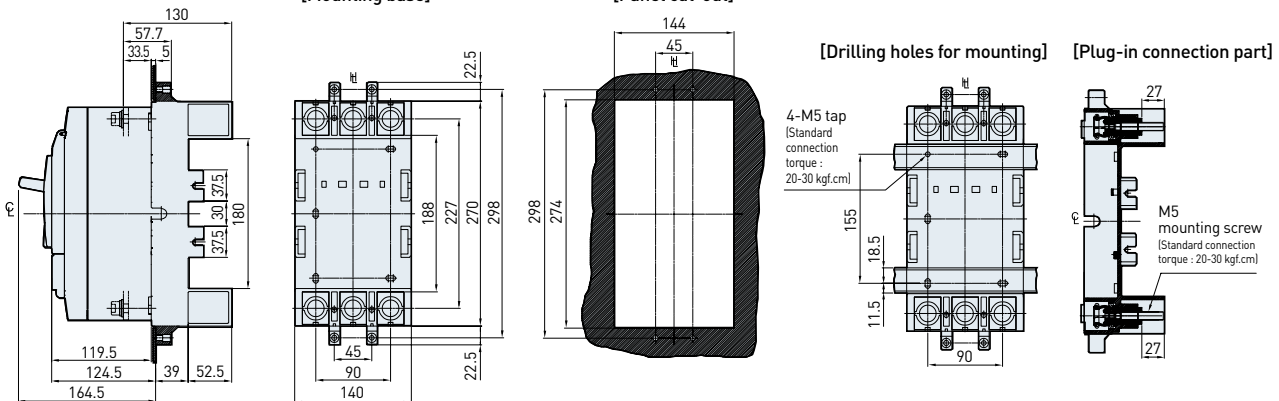
[Mounting base]
