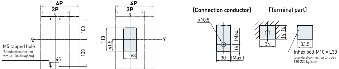
[Drilling holes for mounting]
